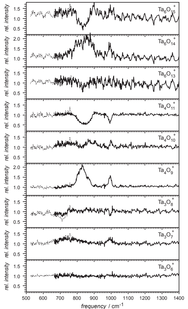
Fig. 2. Ion intensity of tantalum oxide cluster cations as function of IR frequency. The spectra are measured in two overlapping frequency scans that are plotted in different styles. Ion intensities are normalized to the signal in the 1100–1400 \text{cm}^{-1} range.
