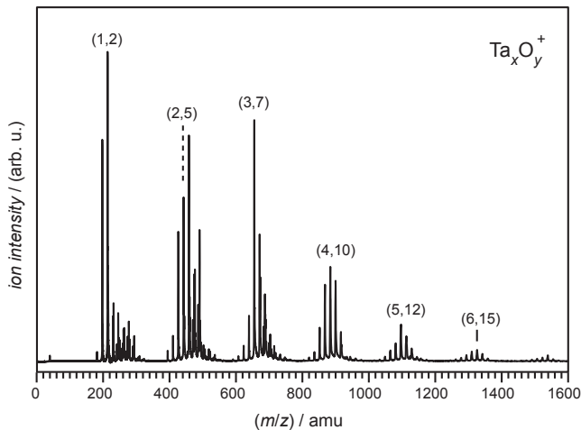
Fig. 1. Mass spectrum of tantalum oxide cluster cations. Dominant oxide cluster peaks are marked with their corresponding stoichiometry ( x, y ). The distribution shows additional signals that can be assigned to hydrates and carbon containing clusters.
