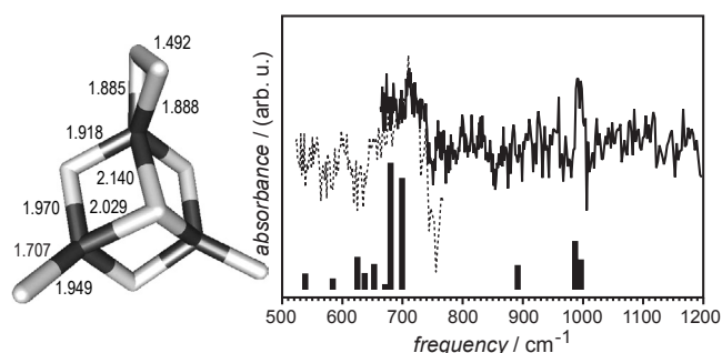
Fig. 3. Structure of \text{Ta}_3\text{O}_8^+ ( C_s sym.) and comparison of experimental and calculated IR spectrum. The structure has been optimized with DFT (B3LYP, LACVP* basis set) using Jaguar 4.0 [22]. The wavenumber axis of the calculated IR spectrum has been linearly scaled to give overlap with the experimental Ta=O stretch frequency resulting in a scaling factor of 0.96.
